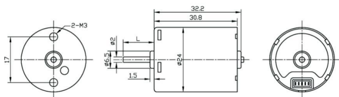
Gear Motor Dimensions (mm)
