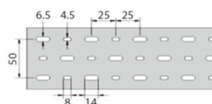
Bottom with triple holes for width over 75mm
