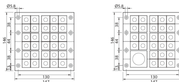
CES 2ET triple row cable entry frame
