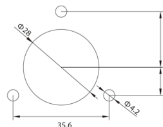
DIMENSION (mm)
