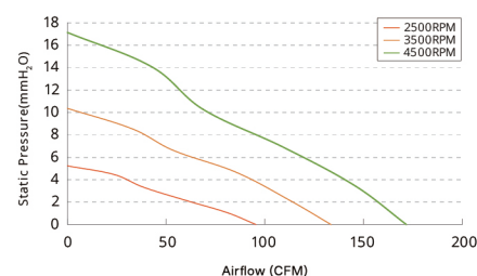
Air Performance
