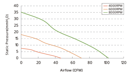
Air Performance
