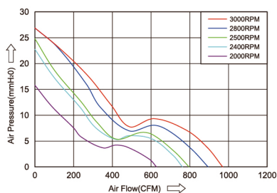
Air Performance
