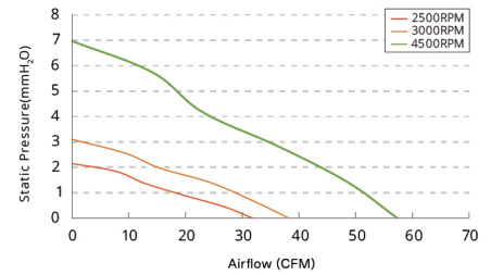
Air Performance
