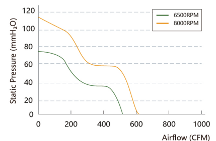
Air Performance
