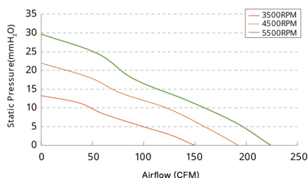
Air Performance
