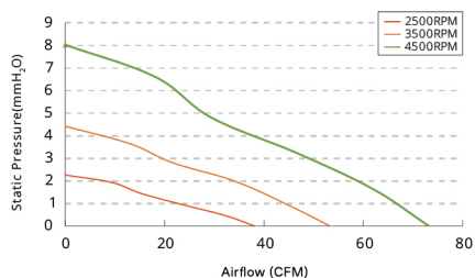
Air Performance
