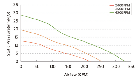
Air Performance
