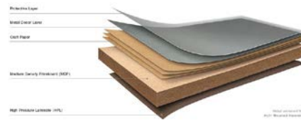
MDF core
