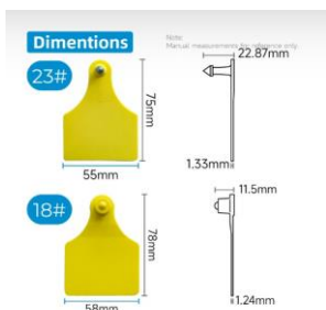
ITEM-30 Tamper proof Calf Tag: 23#+18#
