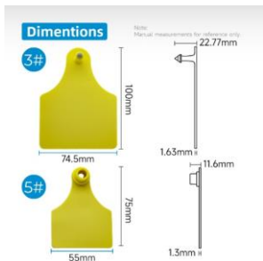
ITEM-27 Medium+Maxi Size Cow Tag: 3#+5#
