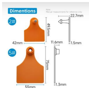
ITEM-26 Small+Medium Size Calf Tag: 2#+5#
