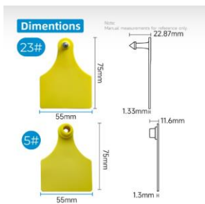
ITEM-29 Two Medium Size Calf Tag: 23#+5#
