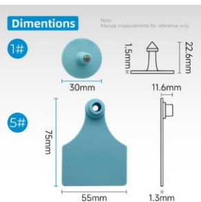
ITEM-15 Medium Size Calf Tag: 1# + 5#
