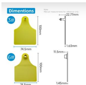
ITEM-28 Two Maxi Size Cow Tag: 3#+6#
