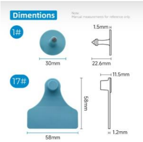
ITEM-7 Pig/Goat Tamper proof Tag Pro: 1#+17#
