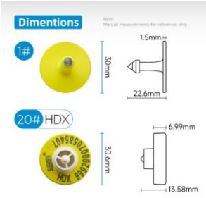
ITEM-36 Tamperproof Ultra Cap EID Tag 1#+20# HDX
