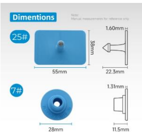
ITEM-10 Swine Tag: 25#+7#
