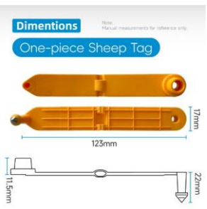
ITEM-14 Goat/Lamb One-Piece Type Ear Tag
