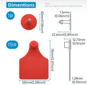
ITEM-21 Calf Tamper proof Tag Pro: 1#+19#
