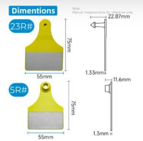
ITEM-24 Two Medium Size Reflective Tag: 23(R)#+5(R)#
