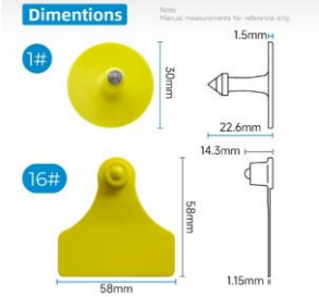
ITEM-6 Pig/Goat Tamper proof Tag: 1#+16#
