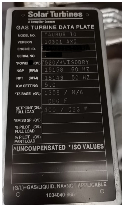
Nameplate of the turbine
