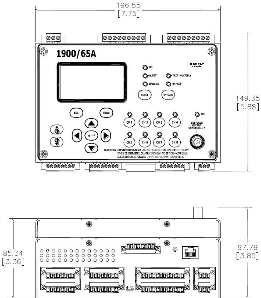
Figure 3: Combined Dimensions
