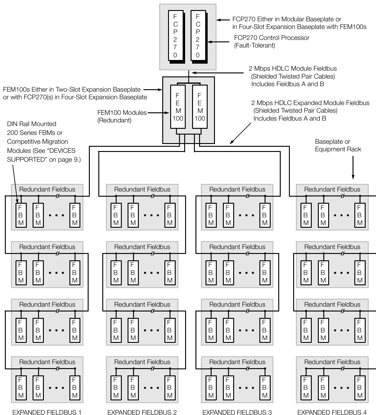
Figure 3. Typical Expanded Fieldbus Network Configuration (Simplified) With Four Expanded Baseplate Groups
