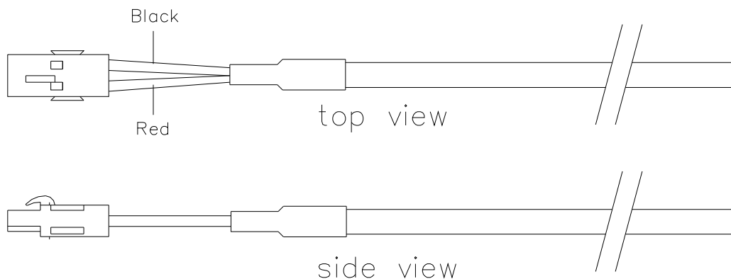
Figure 518 Layout of the FS-PDC-FTA24 power distribution cable
