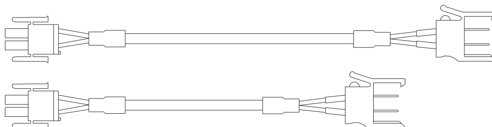
Figure 507 Layout of the FS-PDC-CPSET power distribution cables
