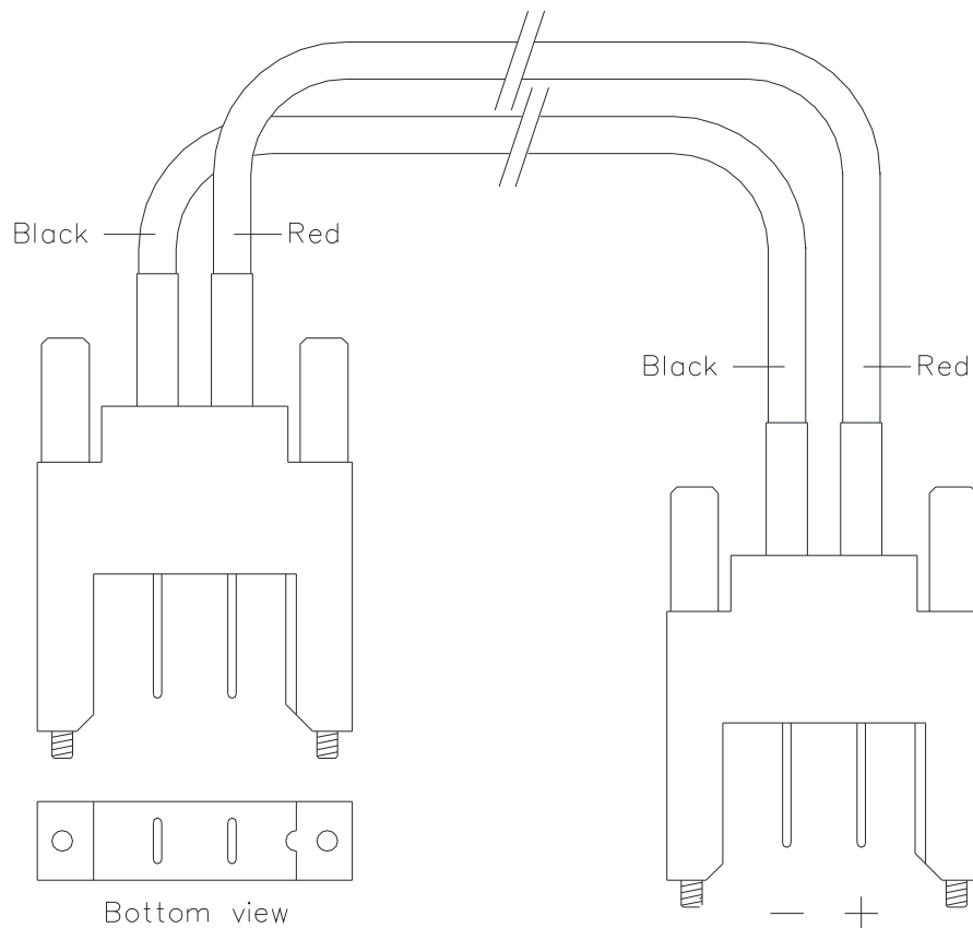
Figure 504 Layout of PDC-MBMB-1 power distribution cable
