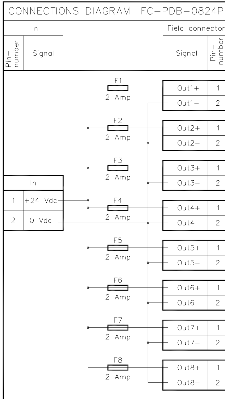
Figure 503 Connection diagram
