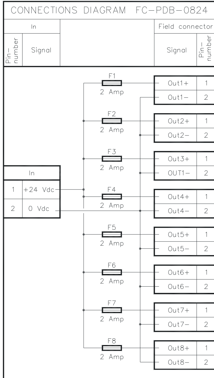
Figure 499 Connection diagram
