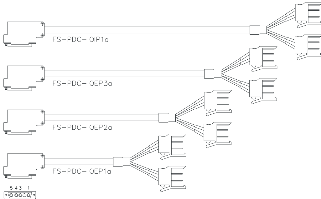
Figure 509 Layout of the FS-PDC-IOSET power distribution cables
