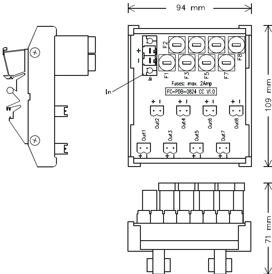
Figure 496 PDB-0824 board layout
