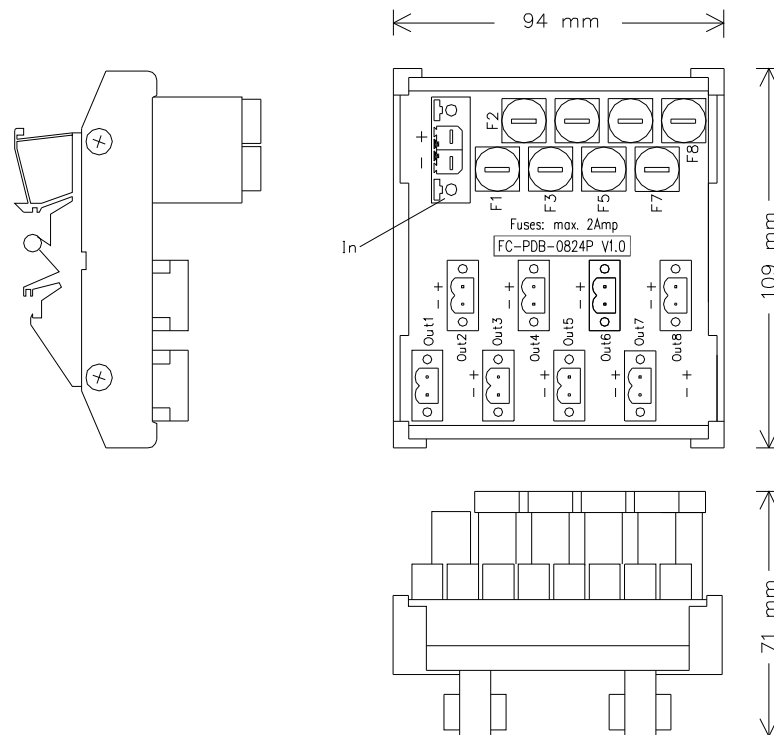
Figure 500 PDB-0824P board layout
