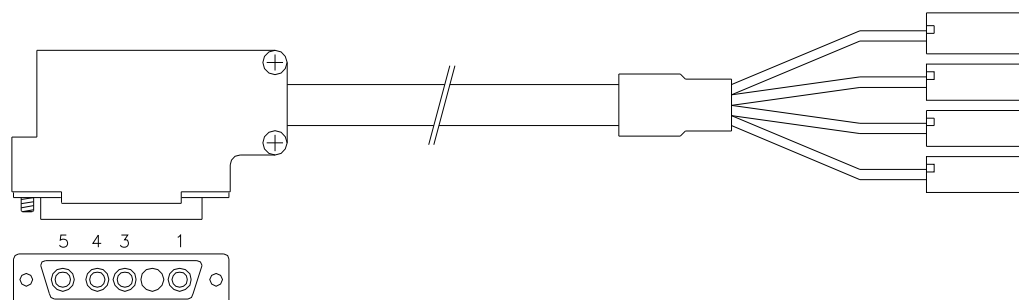
Figure 513 Layout of the FS-PDC-IOxPx power distribution cables
