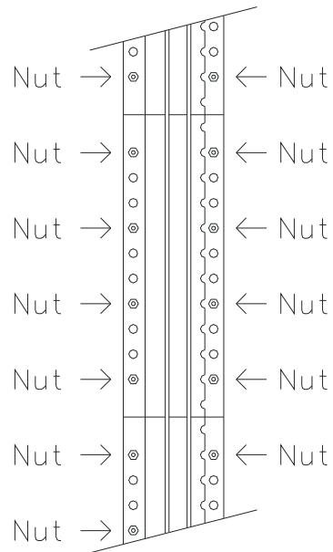
Figure 505 Section of the MB-0001 mains power rail
