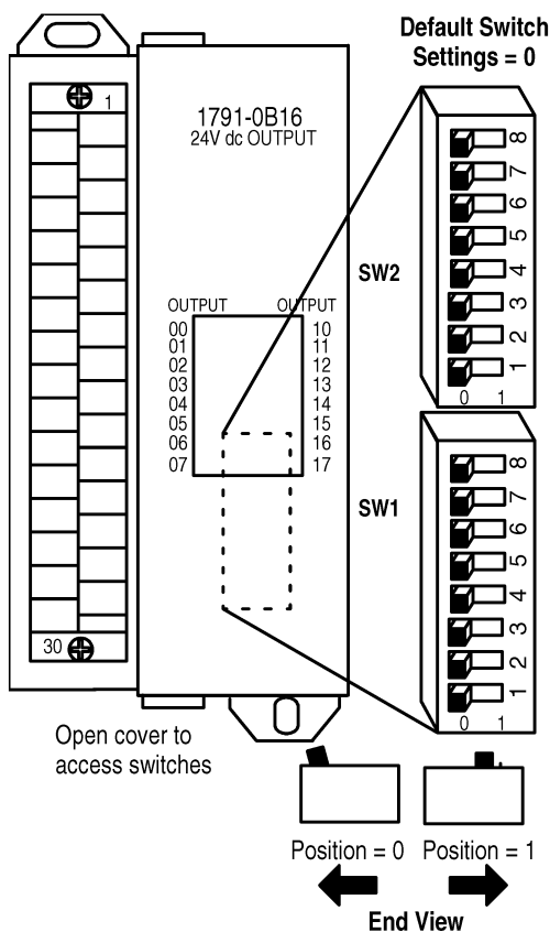
Figure 6 Switch Settings
