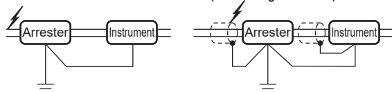
(1) Interconnect Grounding (2) Interconnect Grounding (when using shield line)
