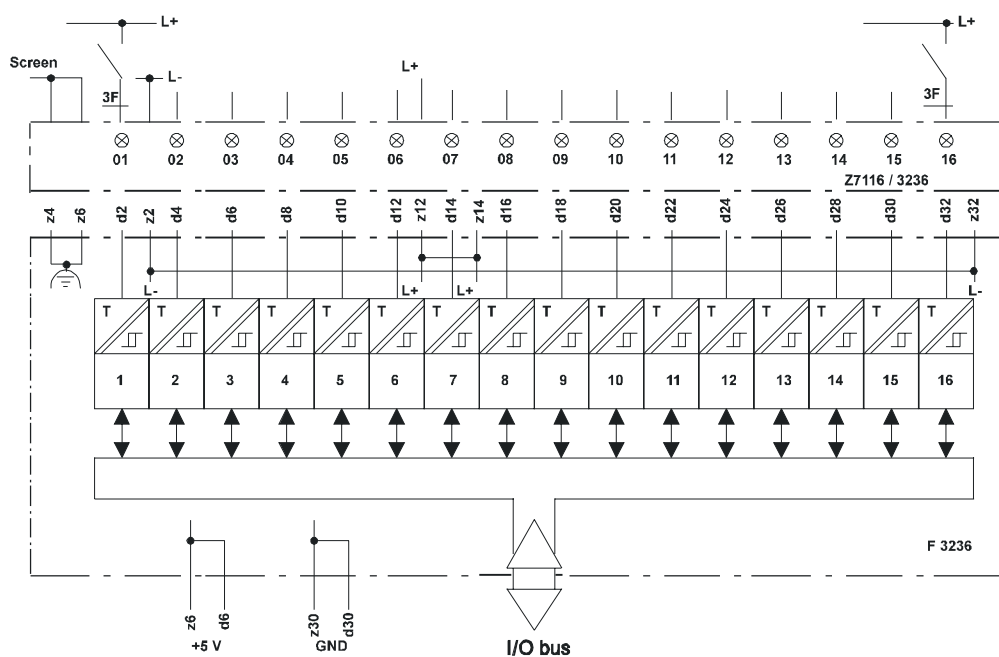
Block diagram
