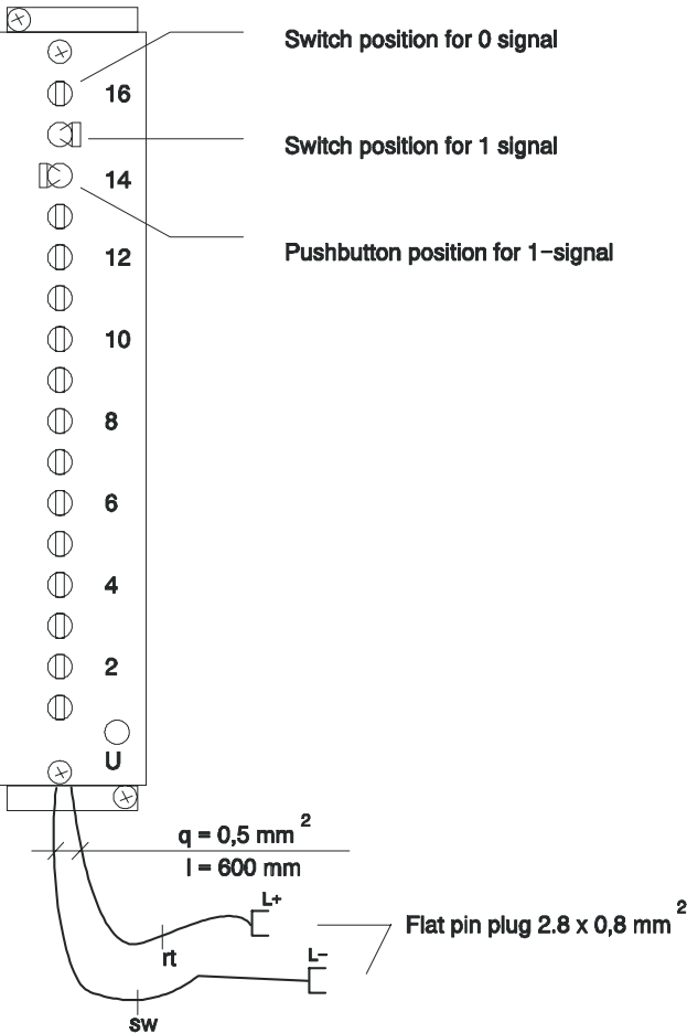
Test plug diagram Z 7201 / 3236
