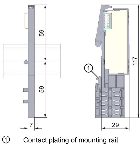
Figure A-1 Dimensional drawing of the server module
