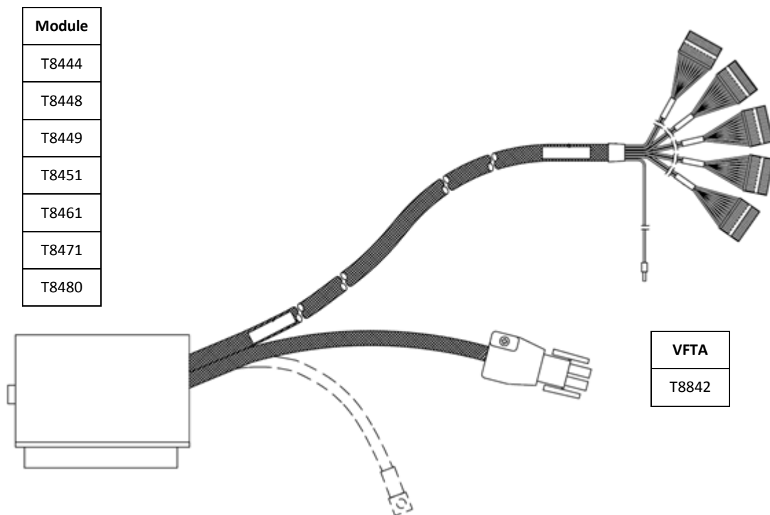
Figure 10 I/O SmartSlot Cable Type TC-510
