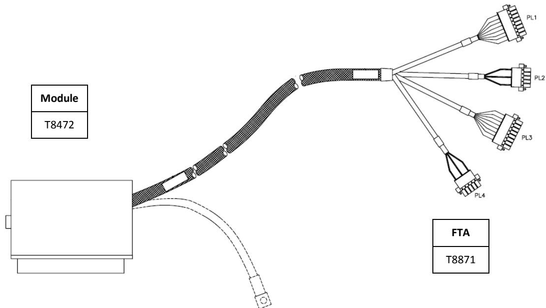
Figure 16 I/O SmartSlot Cable Type TC-521
