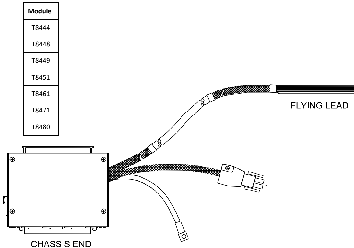
Figure 8 I/O SmartSlot Cable Type TC-508
