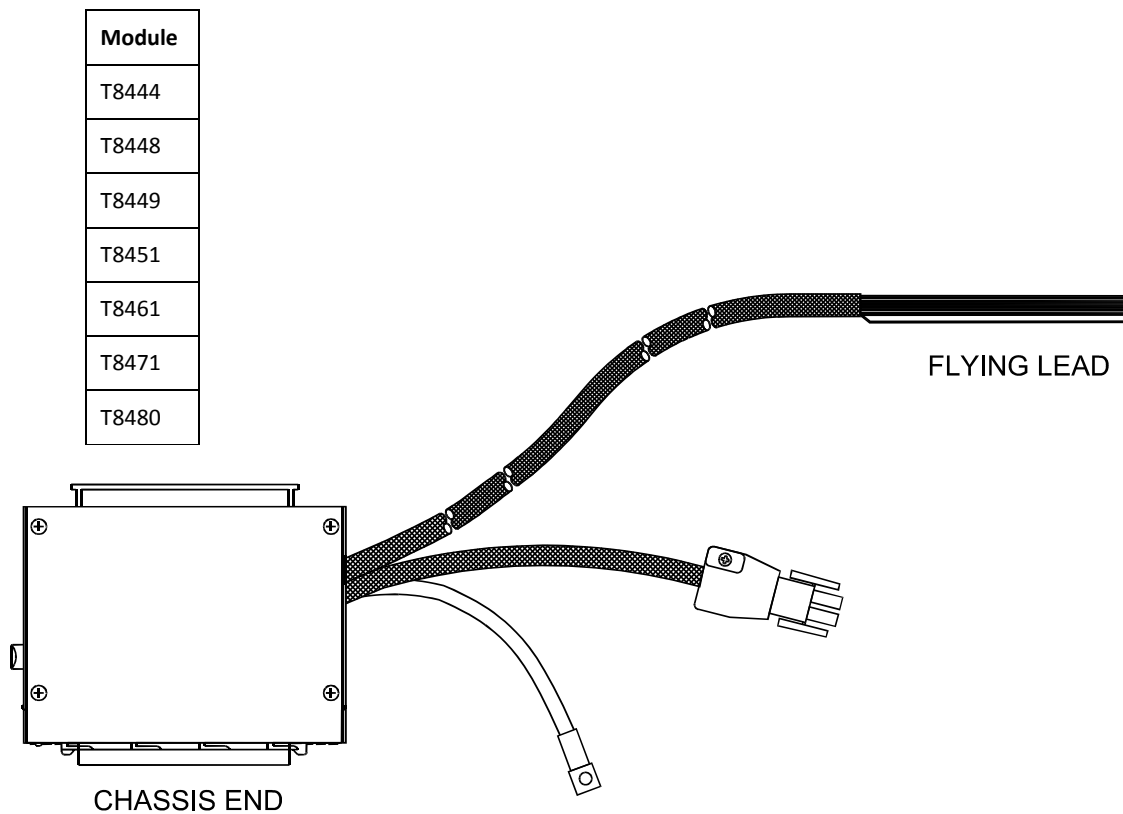
Figure 6 I/O SmartSlot Cable Type TC-506
