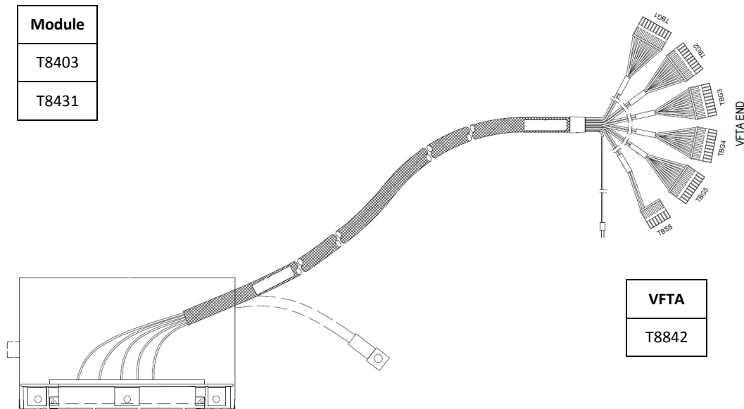
Figure 11 I/O SmartSlot Cable Type TC-511
