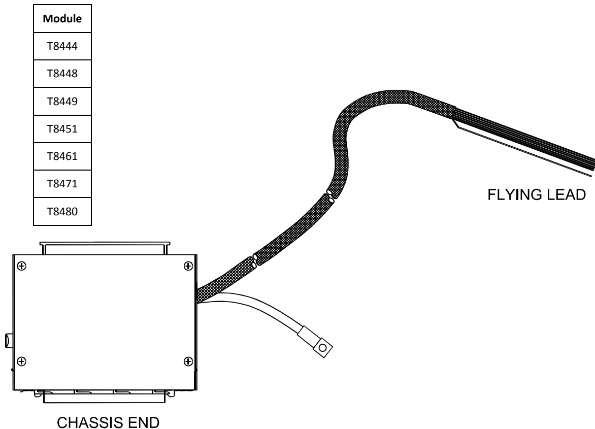
Figure 13 I/O SmartSlot Cable Type TC-516
