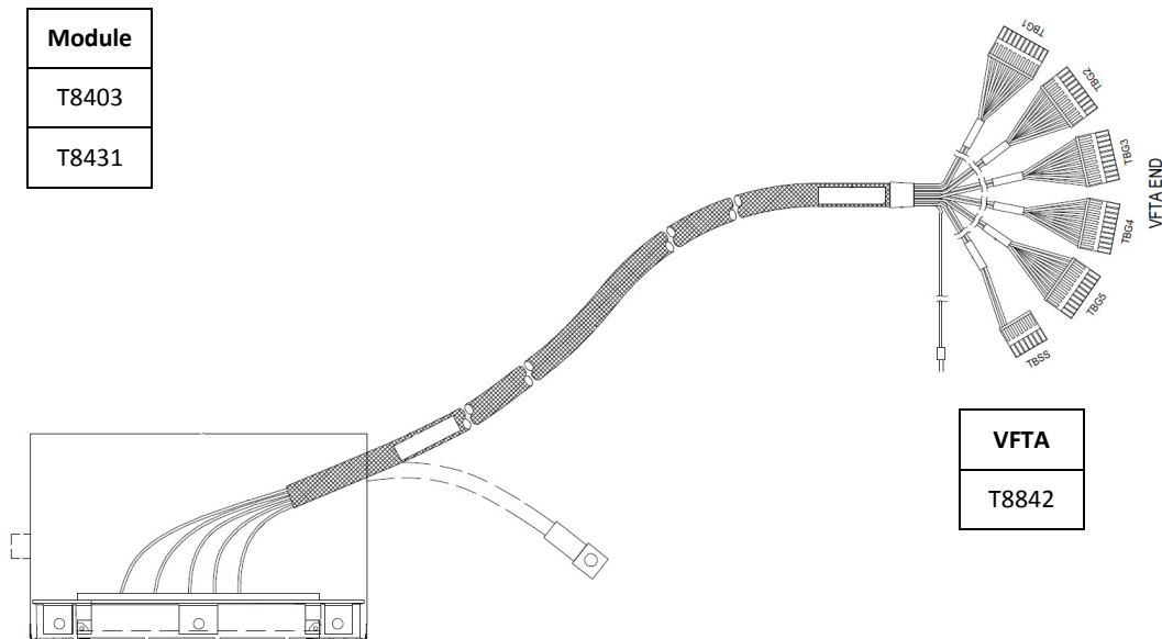
Figure 12 I/O SmartSlot Cable Type TC-512
