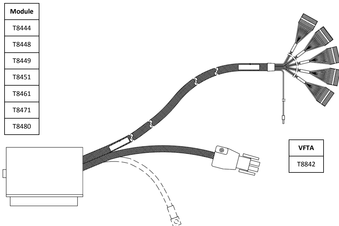
Figure 9 I/O SmartSlot Cable Type TC-509
