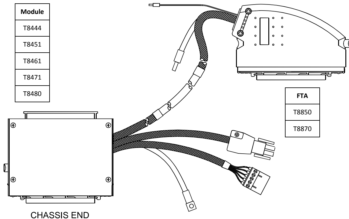
Figure 7 I/O SmartSlot Cable Type TC-507
