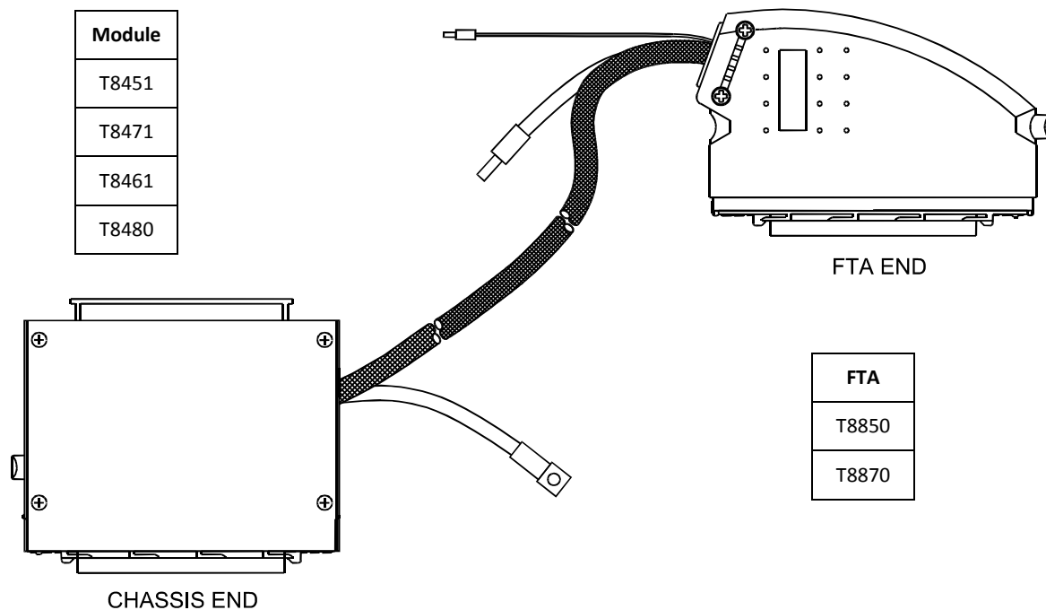
Figure 14 I/O SmartSlot Cable Type TC-517
