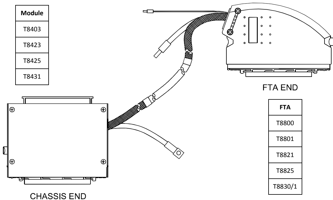
Figure 3 I/O SmartSlot Cable Type TC-503
