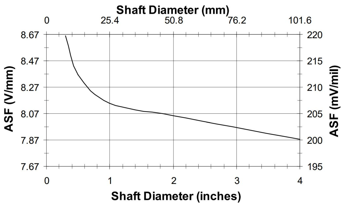
Figure 13: Radial Sensitivity to Shaft Size
