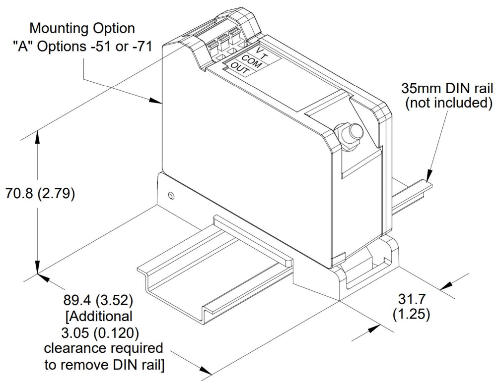
Figure 23: DIN Mount 3300 XL NSv Proximitior Sensor
