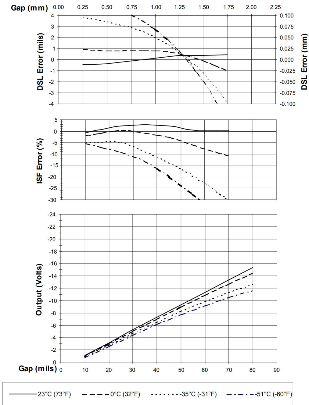
Figure 3: Typical 3300 NSv Probe + 1m Cable @ Low Temperature (Proximitor Sensor + 4 m of Extension Cable @ 25°C)
