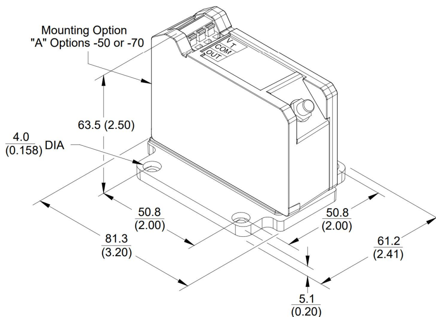
Figure 22: Panel Mount 3300 XL NSv Proximitior Sensor
