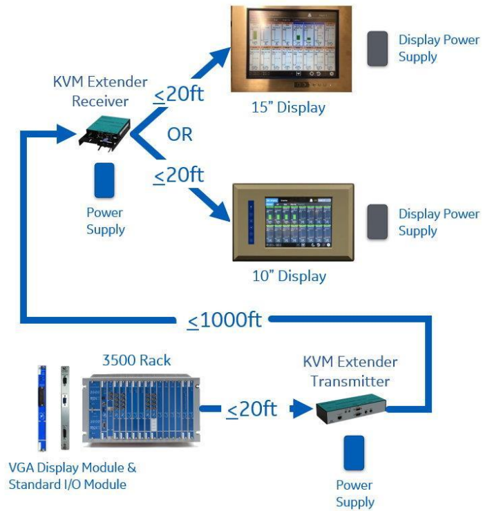
Figure 4: Single Rack with KVM Extender
