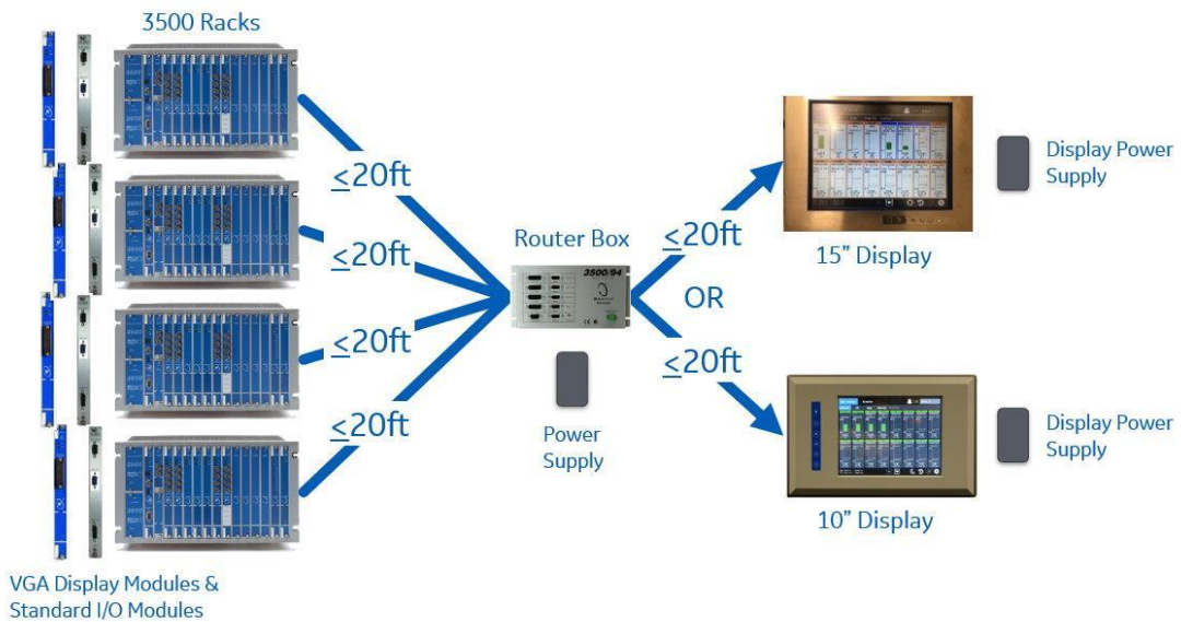
Figure 5: Multiple Racks with Router Box
