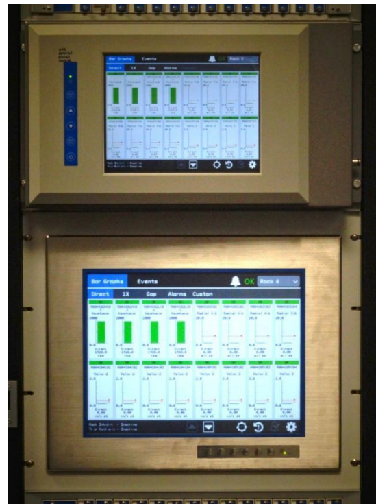
10" Display Face Mount option (upper), 15" Display 19" EIA Rack Mount option (lower)
