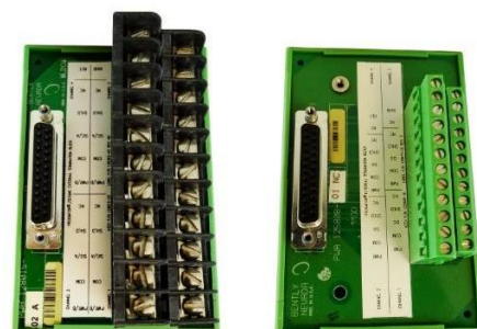
ET Blocks with screw terminals for lugged field wiring (left) and high-density "Euro" connectors for non-lugged field wiring (right)
