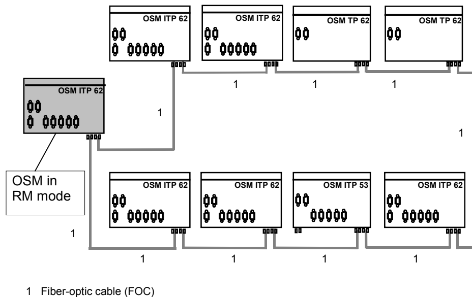
Figure 12: Redundant Ring Structure with OSMs
