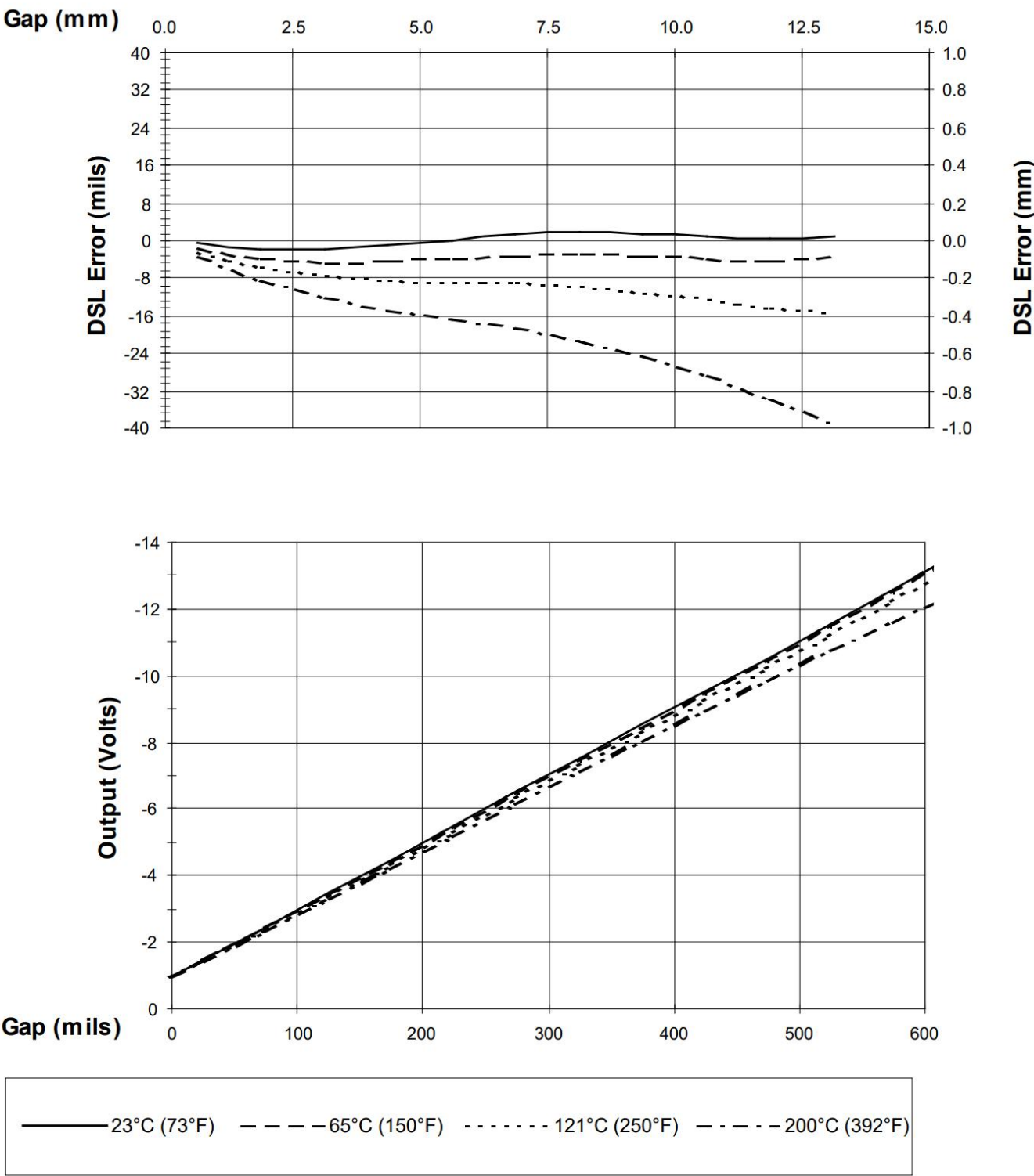
Figure 4: Typical 3300 XL 25mm Probe + 1m Cable @ High Temperature (Proximitior Sensor + 4m of Extension Cable @ 25 °C)
