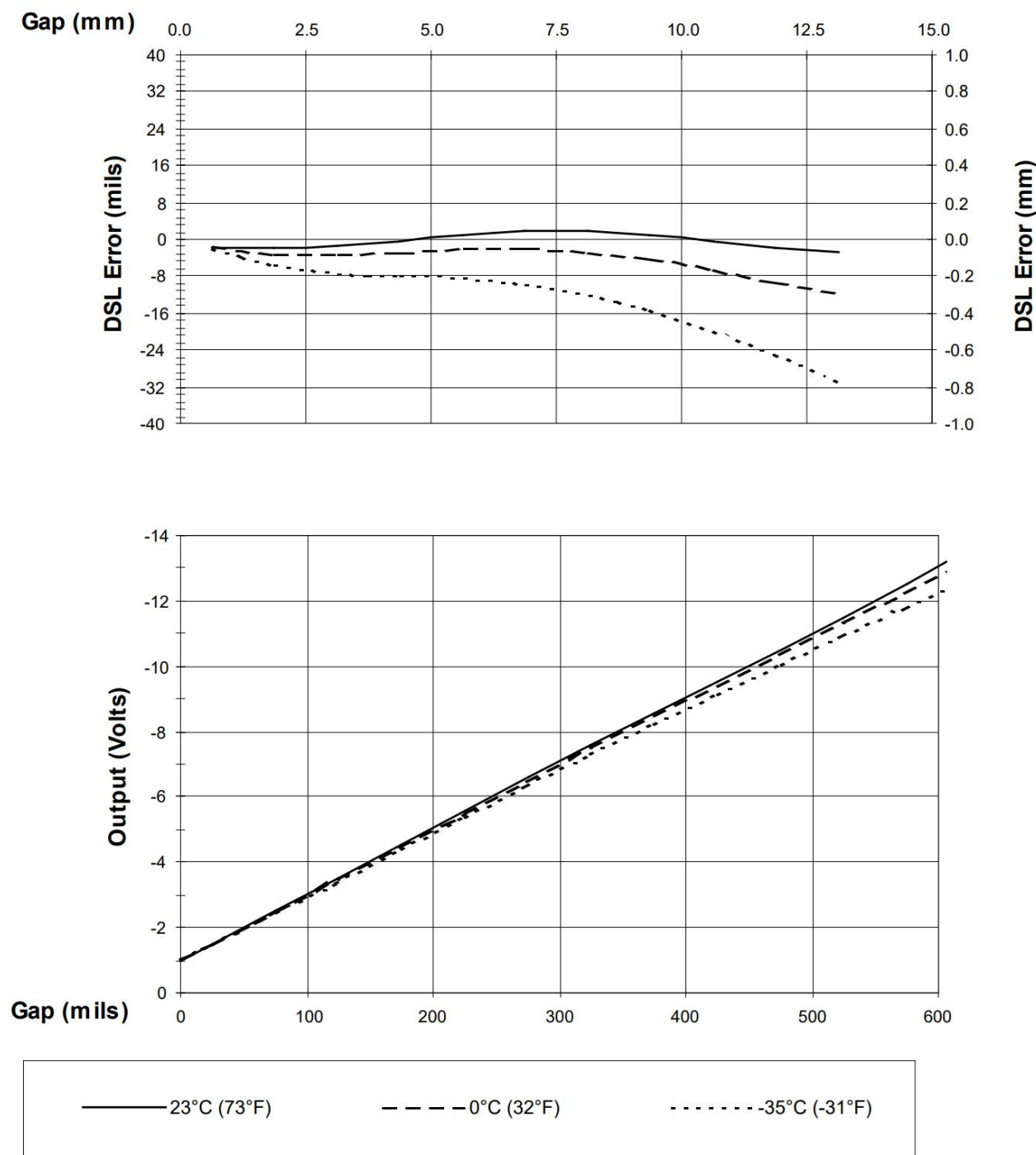
Figure 7: Typical 3300 XL 25mm 9m Proximitor Sensor with 8m of Extension Cable @ Low Temperature (Probe is at 25°C)
