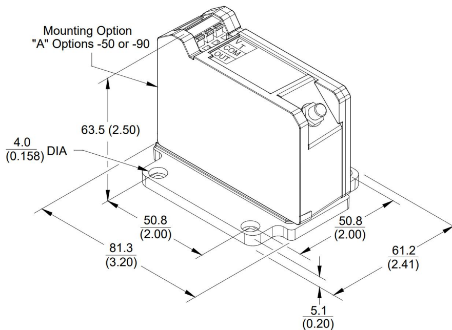
Figure 18: 330850 Panel Mount 3300 XL 25mm Proximitior Sensor
