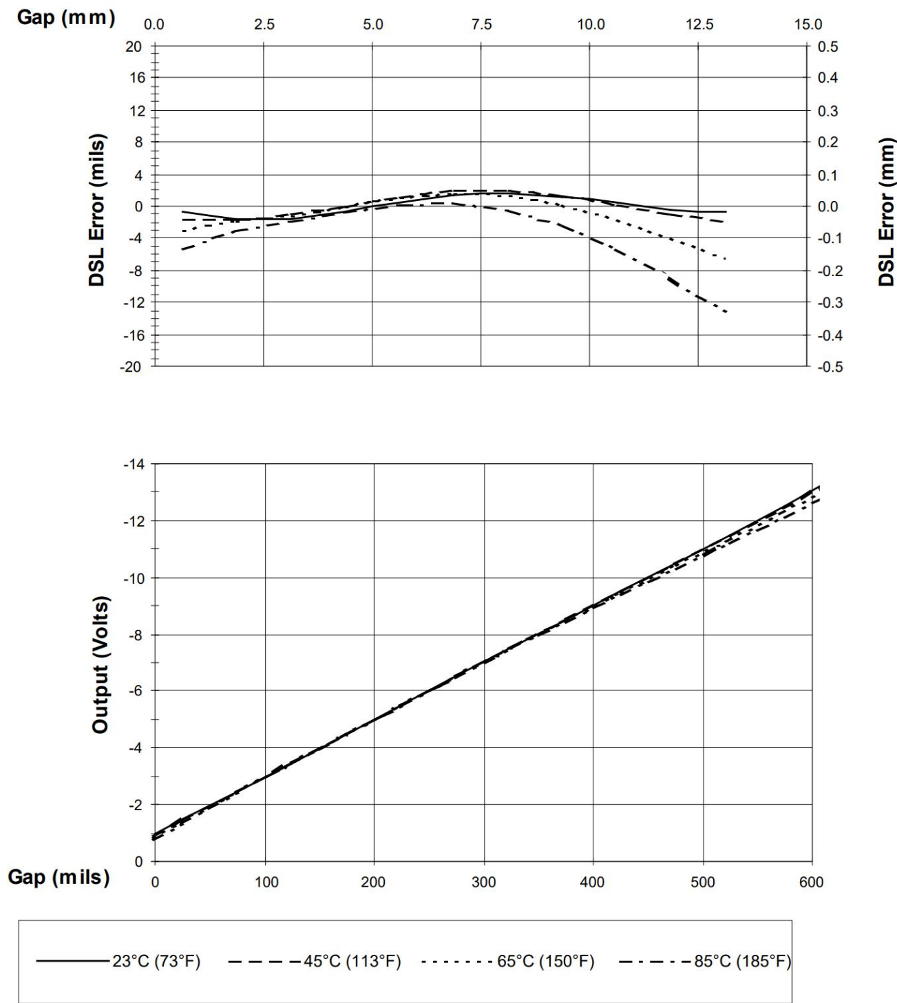
Figure 6: Typical 3300 XL 25mm 5m Proximitior Sensor with 4m Extension Cable @ High Temperature (Probe is at 25°C)
