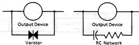
Surge Suppression for Inductive AC Output Devices
