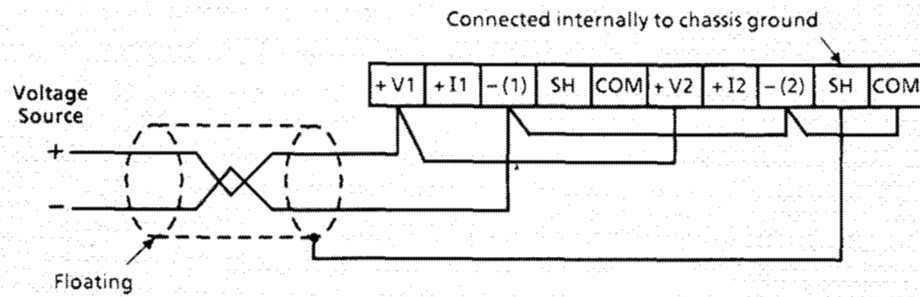
1. Voltage source, single ended connection.
