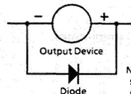
Surge Suppression for Inductive DC Output Devices
