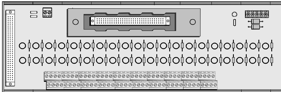
Figure 1 T8830 Layout
