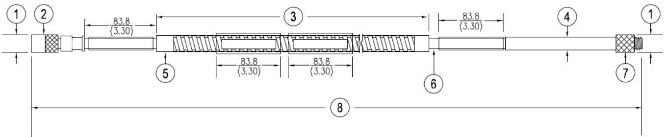
Figure 4: Installed Connector Protectors
