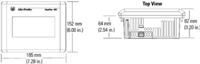
Dimension Diagram
