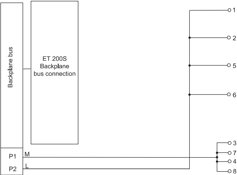
Figure 1-1 Block diagram of the 4POTDIS
