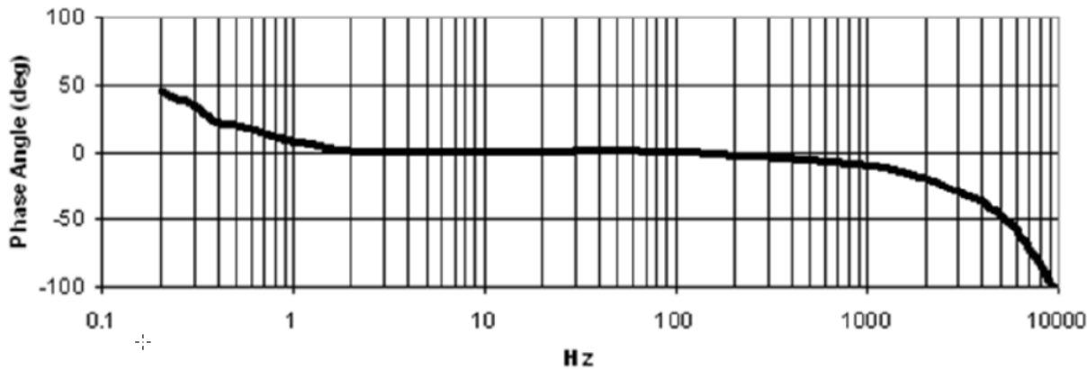
Figure 3 - 6: 200355 Accelerometer Phase
