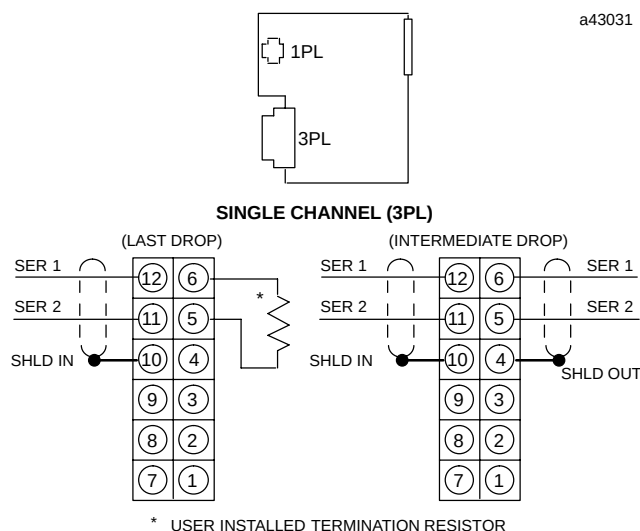
Figure 5. Wiring Diagram
