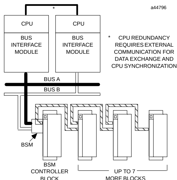
Figure 6. Dual Bus System
