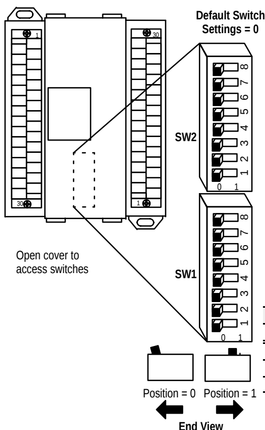
Figure 6 Switch Settings
