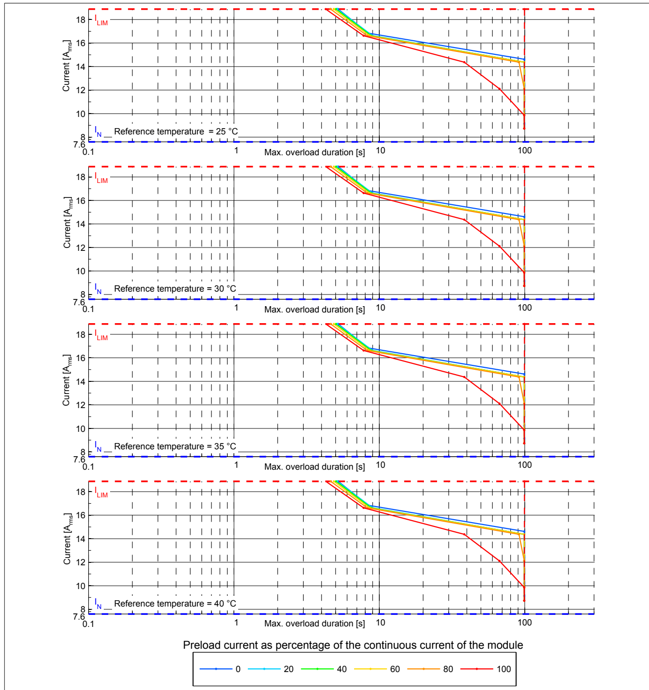
Figure 1: 8BVI0055HWDx.000-1 - Overload characteristics, overload response - WARNING
