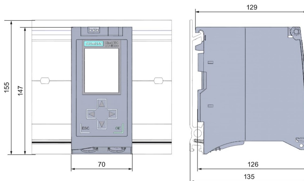
Figure A-1 Dimensional drawing of the CPU 1515T-2 PN, front and side view
