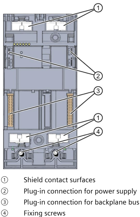
Figure 2-4 View of the CPU 1515T-2 PN - rear
