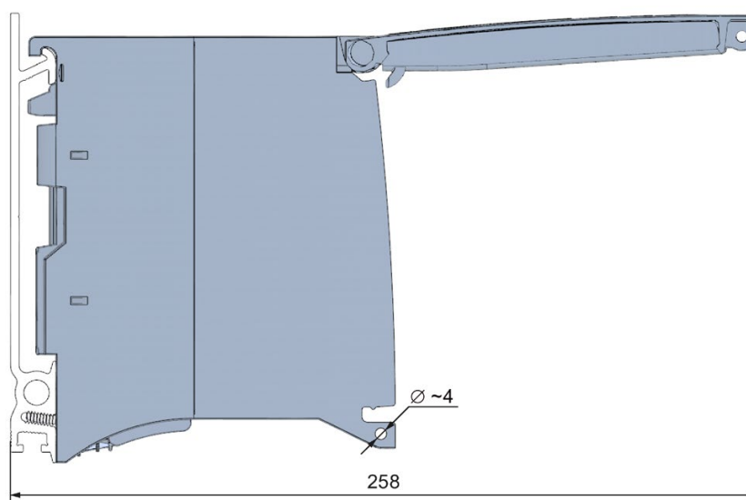
Figure A-2 Dimensional drawing of the CPU 1515T-2 PN, side view with open front panel
