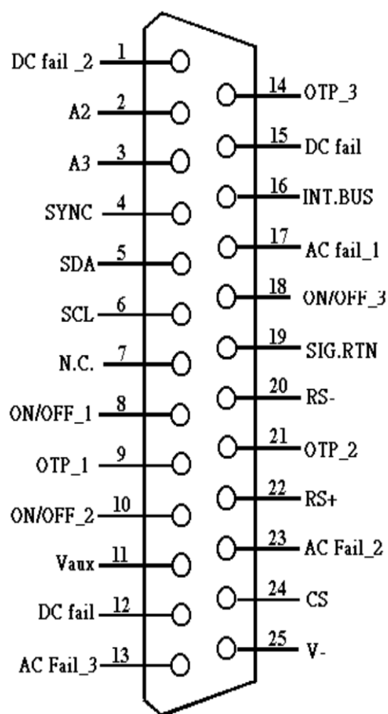
Figure 5 Interface Connector
