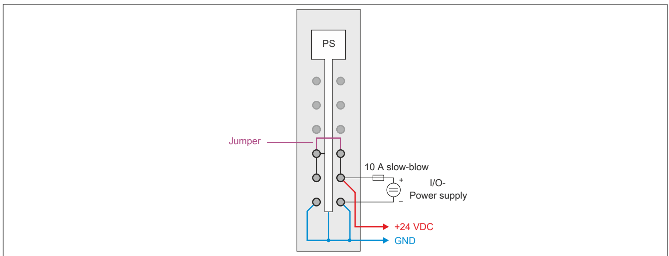
Figure 7: X20 CPUs - Connection example with a supply and jumper
