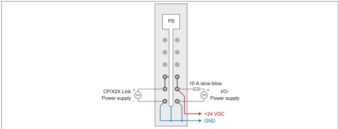
Figure 6: X20 CPUs - Connection example with two separate supplies
