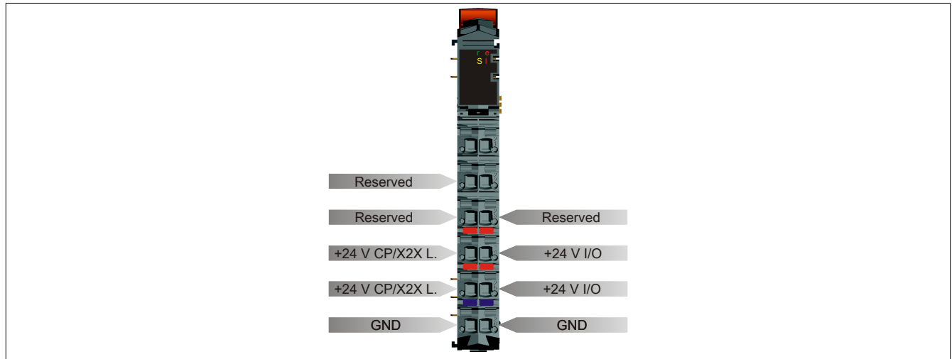
Figure 5: X20 CPUs - Pinout - Integrated power supply
