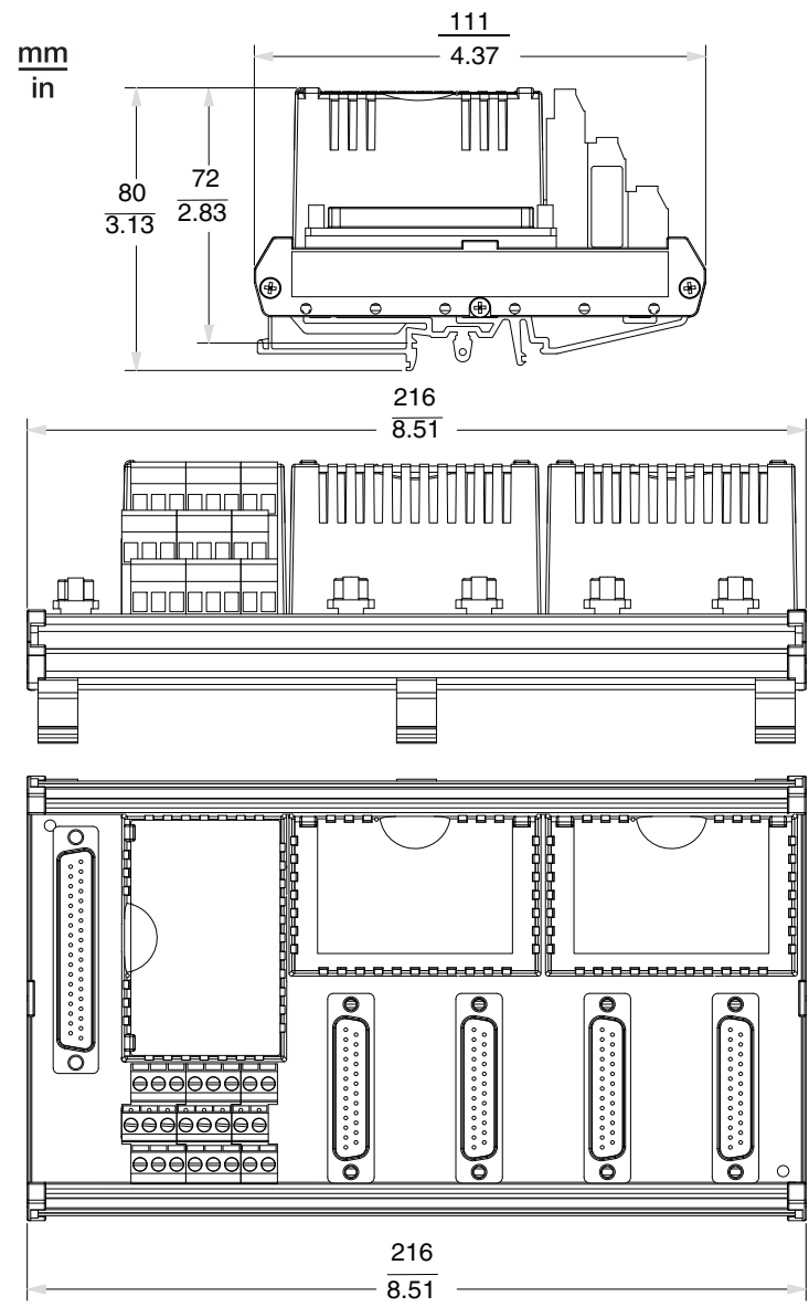
Compression Screw Termination Assembly (P0926GH)
