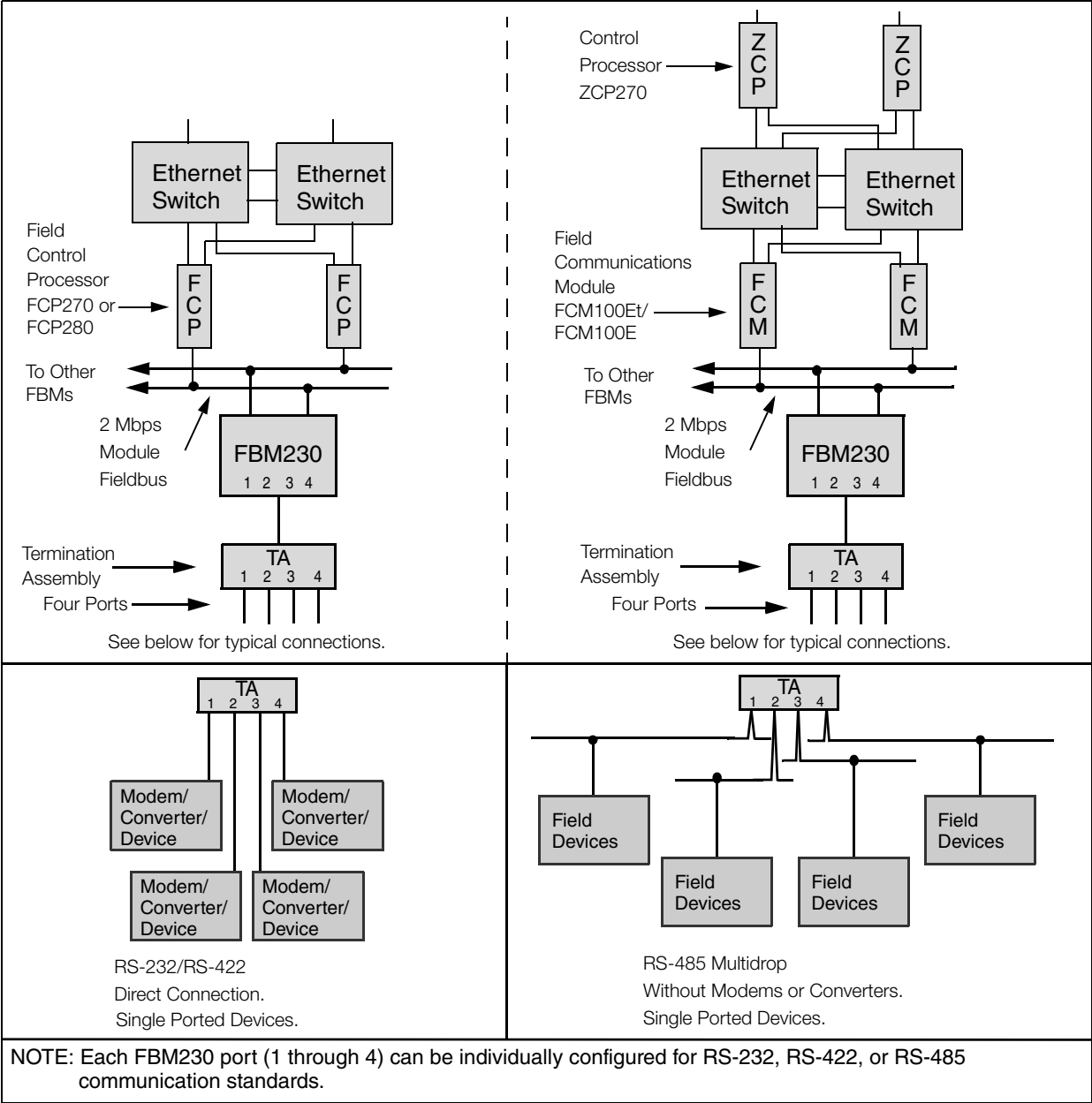
Figure 1. FBM230 in Typical Network Configurations
