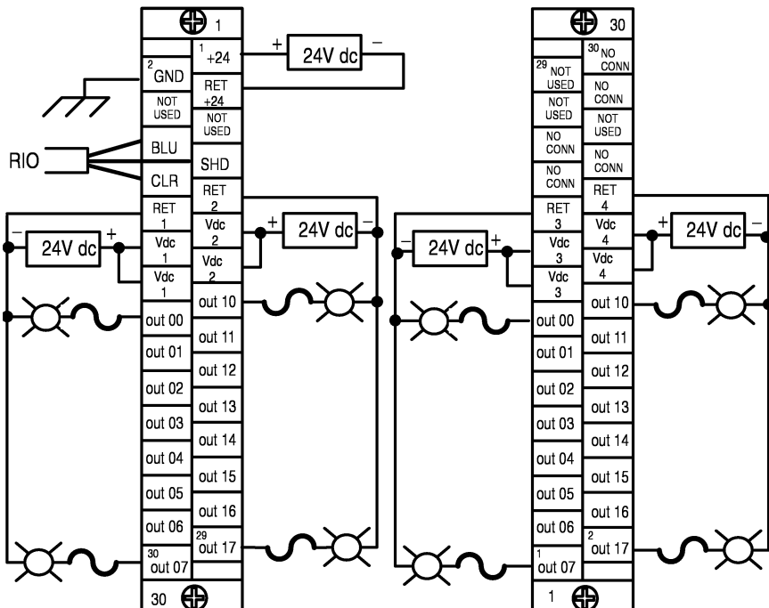
Figure 4 Wiring Connections with PLC Family Programmable Controllers (refer to Table B)
