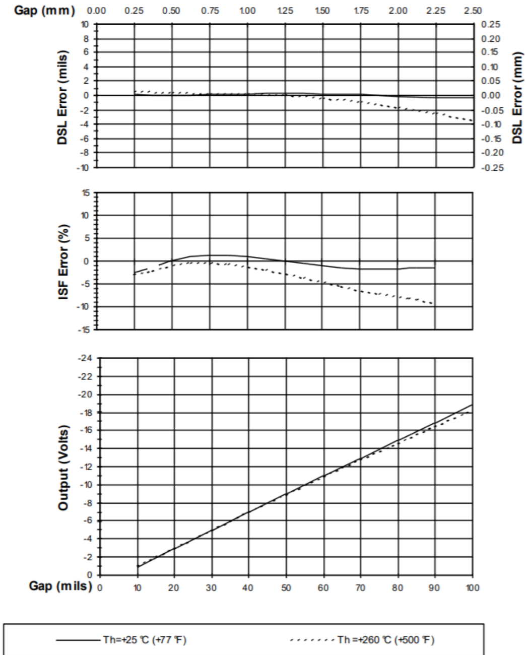
Figure 8: Typical 3300 XL Extended Temperature Range Probe and 4 m Extended Temperature Range Extension Cable at T_h (Proximito Sensor and Probe Tip with 1-foot Cable are at +25\text{ }^{\circ}\text{C} )
