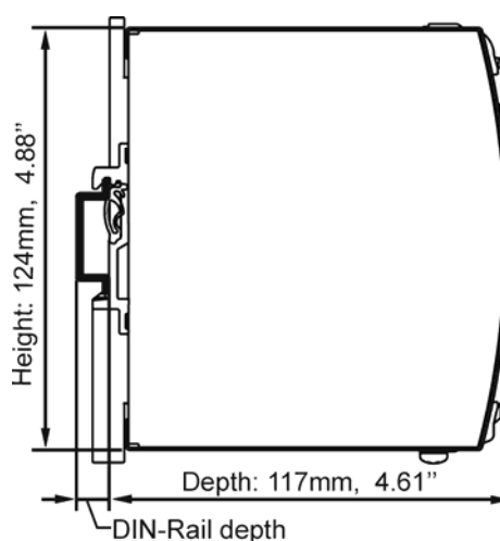
Fig. 24-2 Side view
