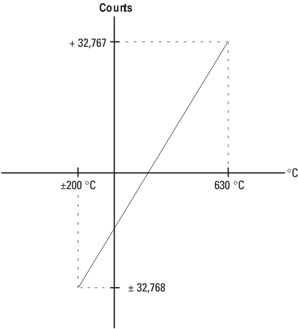
Linear Relationship Between Temperature and Proportional Counts
