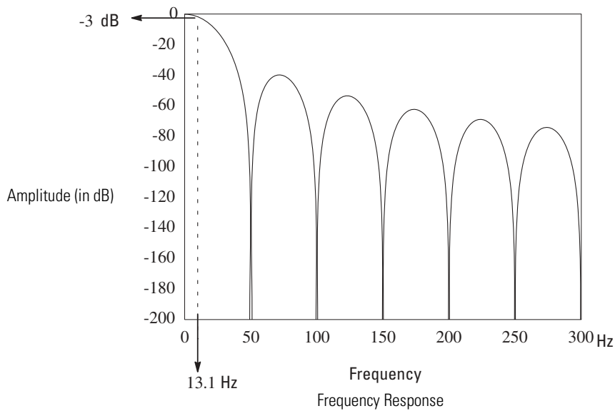
60 Hz Filter Notch Frequency
