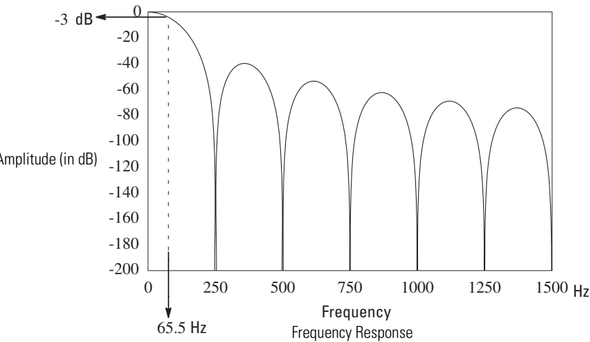
250 Hz Filter Notch Frequency
