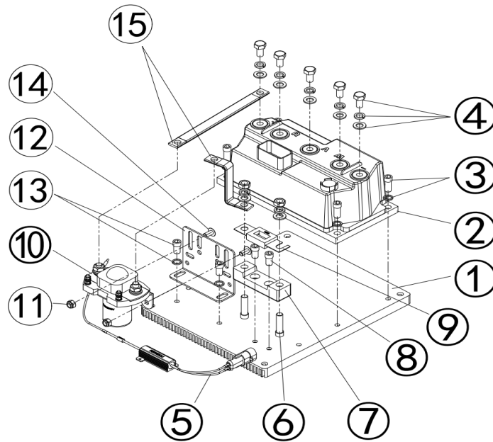
2.3 Controller Assembly (Ec 电控总成)
