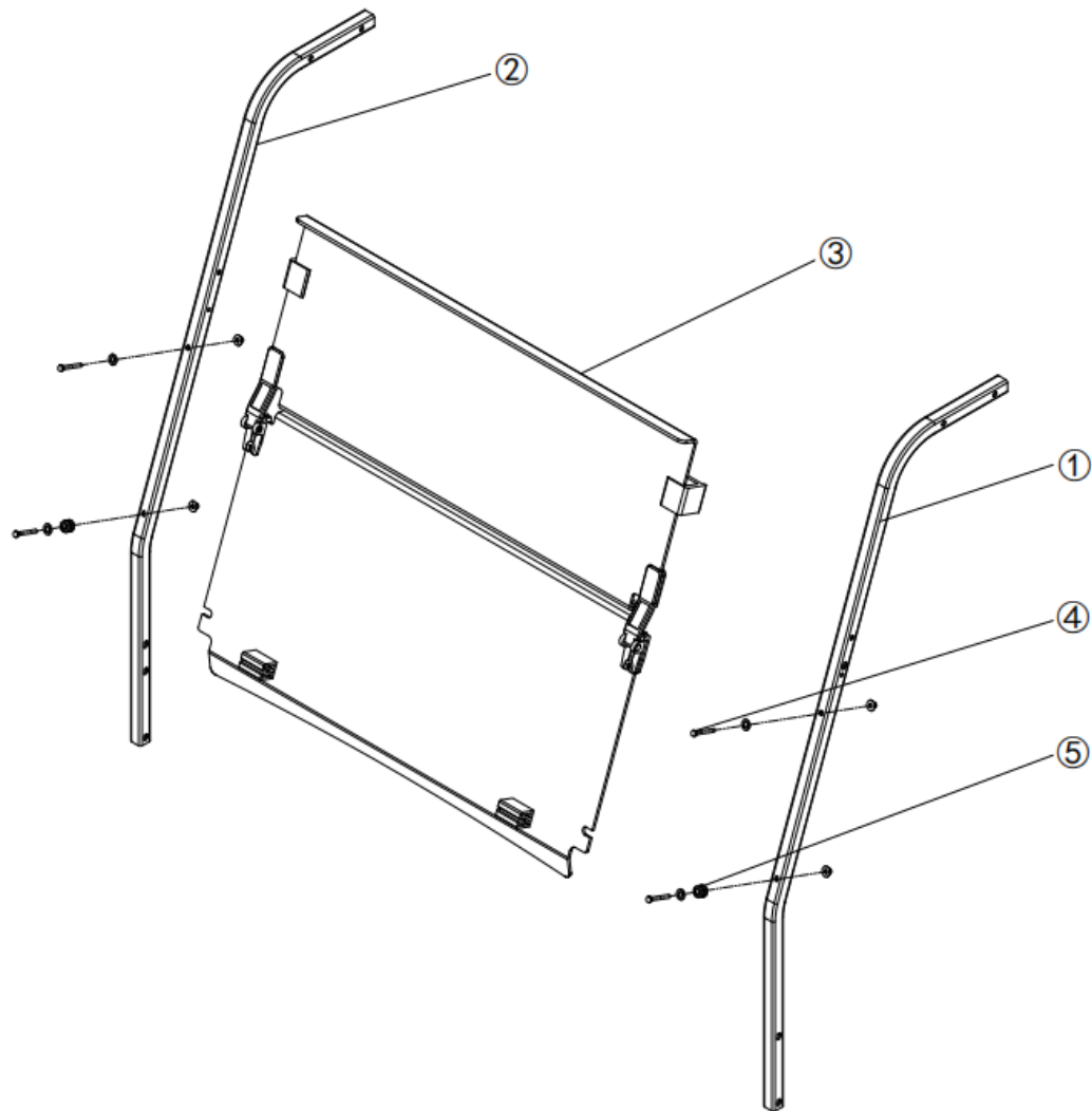
3.7.2 Hinge Type Split Front Windshield (铰链式折叠前风挡总成)
