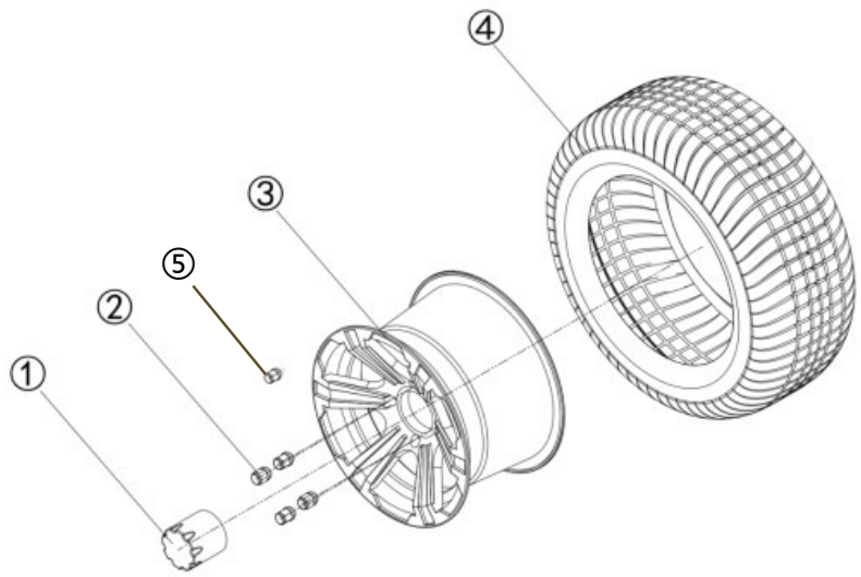
1.6 Wheel (CF 轮胎总成)
