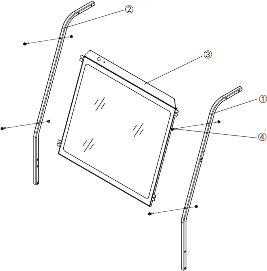
3.7.3 Laminated Glass Windshield (夹胶前风挡总成)
