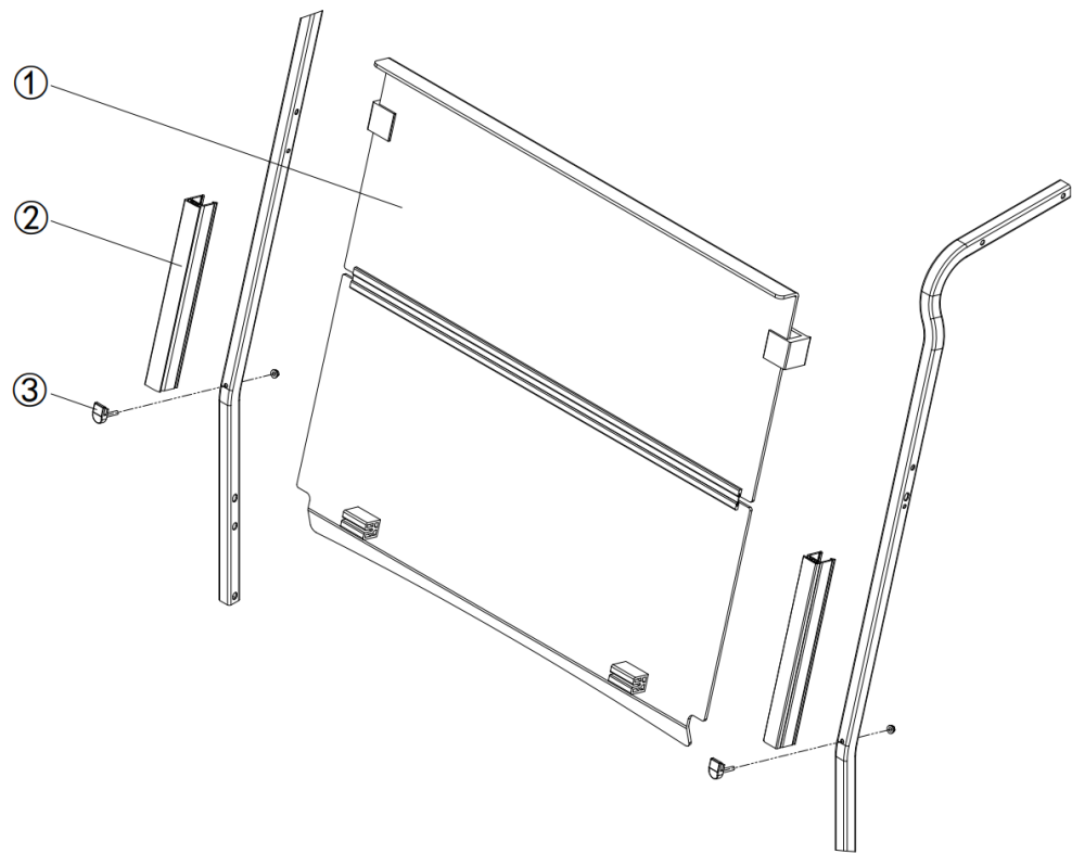
3.7.1 Split Front Windshield (折叠前风挡总成)
