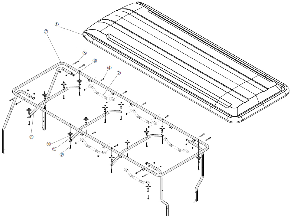
3.8.6 6P Roof (6 座顶棚总成)
