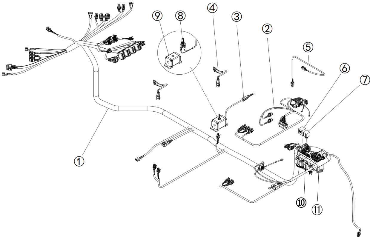
2.1 Wiring Harness (Ea 线束总成)
