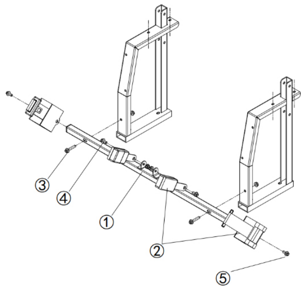
3.9.1 Front 2-point Seatbelt (BL 安全带总成)
