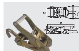
BTRB030 50MM WITH J HOOK CAP: 5,000 kgs
