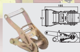
BTRB023 2" WITH ALUM MED WIDE HANDLE CAP: 5,000 kgs / 11,000 lbs.
