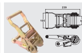
BTRB032 2" WITH WIDE HANDLE CAP: 8,000 kgs / 17,600 lbs.
