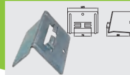
2"Corner Protector(Steel) Weight=0.304kg
