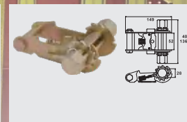
BTRB022 2" WRENCH-OPERATED CAP: 4,545 kgs / 10,000 lbs.
