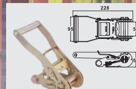
BTRB021 2" WITH ALUM LONG WIDE HANDLE CAP: 6,000 kgs / 13,200 lbs.
