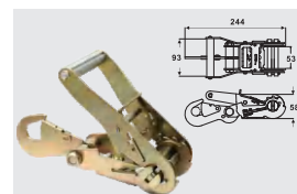
BTRB027 W/ F081-A CAP: 3,000 kgs / 6,600 lbs BTRB028 W/ F082-A CAP: 5,000 kgs / 11,000 lbs
