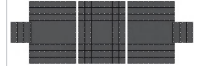
Ends: 20' x 18' Drop/Flap: 6' Middle: 20' x 18' Drop/Flap: 6'
