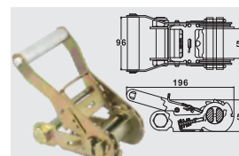
BTRB031 2" WITH WIDE HANDLE CAP: 7,000 kgs / 15,400 lbs.
