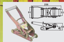
BTRb017 2" ERGO CAP: 5,000 kgs / 11,000 lbs.
