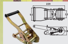
BTRB020 2" WITH PLASTIC HANDLE CAP: 5,000 kgs / 11,000 lbs.
