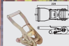
BTRB021 2" WITH ALUM LONG WIDE HANDLE CAP: 6,000 kgs / 13,200 lbs.
