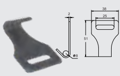
BTSF008 1" NARROW FLAT HOOK, PE COATING CAP: 450 kgs / 1,000 lbs.
