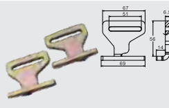
BTFTH003 LEFT HAND BTFTH004 RIGHT HAND 2" SPECIAL SLAT HOOK CAP: 1,363 kgs / 3,000 lbs.
