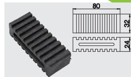
Tire Protector(Rubber or Plastic) 80MMx32 MMx24 MM
