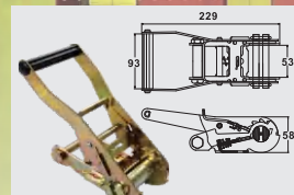
BTRB020 2" WITH PLASTIC HANDLE CAP: 5,000 kgs / 11,000 lbs.
