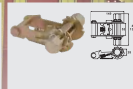
BTRB022 2" WRENCH-OPERATED CAP: 4,545 kgs / 10,000 lbs.
