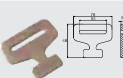
BTFTH011 T HOOK CAP: 3,182 kgs / 7,000 lbs.
