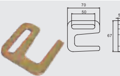
BTFTH002 2" SLAT HOOK CAP: 1,363 kgs / 3,000 lbs.
