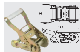
BTRB031 2" WITH WIDE HANDLE CAP: 7,000 kgs / 15,400 lbs.
