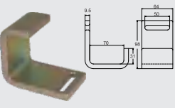
BTSF004 ROLL OFF HOOK CAP: 7,363 kgs / 16,200 lbs.
