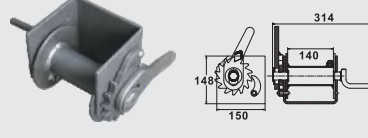
BTBW006 CABLE WINCH, RIGHT HAND BTBW007 CABLE WINCH, LEFT HAND
