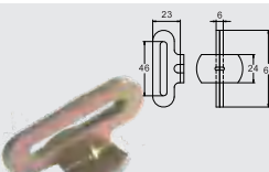
BTFTH007 BUTTERFLY FITTING FOR 25MM HOLE CAP: 909 kgs / 2,000 lb.
