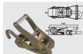
BTRB030 50MM WITH J HOOK CAP: 5,000 kgs
