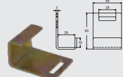
BTSF005 1" FLAT HOOK CAP: 1,000 kgs / 2,200 lbs.
