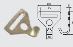
BTFTH001 2" F TRACK HOOK CAP: 1,000 kgs / 2,200 lbs.
