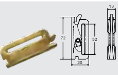
BTFTH008 SPRING LOADED FITTING CAP: 2,727 kgs / 6,000 lbs.
