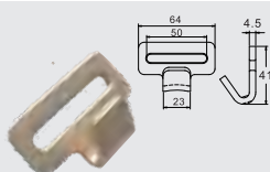
BTFTH005 2" SHORT NARROW FLAT HOOK CAP: 1,800 kgs / 3,960 lbs.
