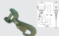
BTSF006 1-3/4" SWIVEL SNAP HOOK CAP: 3,500 kgs / 7,700 lbs.
