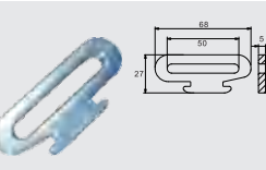
BTFTH010 TRACK FITTING CAP: 1,250 kgs / 2,750 lbs.
