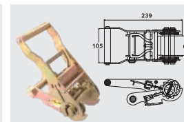
BTRB032 2" WITH WIDE HANDLE CAP: 8,000 kgs / 17,600 lbs.
