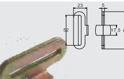
BTFTH006 BUTTERFLY FITTING FOR 19MM HOLE CAP: 680 kgs / 1,500 lbs.
