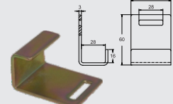
BTSF005 1" FLAT HOOK CAP: 1,000 kgs / 2,200 lbs.
