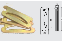
BTFTH009 3-PIECE FITTING CAP: 1,363 kgs / 3,000 lbs.
