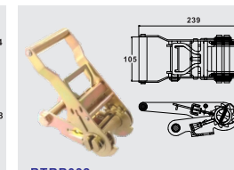
BTRB032 2" WITH WIDE HANDLE CAP: 8,000 kgs / 17,600 lbs.
