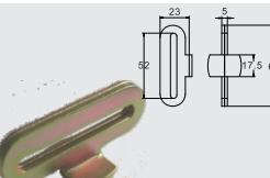
BTFTH006 BUTTERFLY FITTING FOR 19MM HOLE CAP: 680 kgs / 1,500 lbs.
