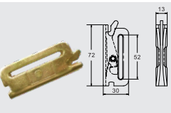
BTFTH008 SPRING LOADED FITTING CAP: 2,727 kgs / 6,000 lbs.
