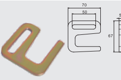
BTFTH002 2" SLAT HOOK CAP: 1,363 kgs / 3,000 lbs.
