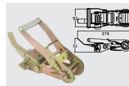
BTRB026 2" WITH ONE WAY BUCKLE CAP: 1,136 kgs / 2,500 lbs.
