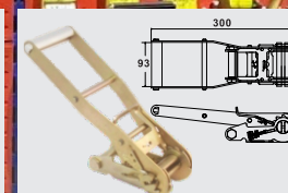
BTRB018 2" EXTRA LONG WIDE HANDLE CAP: 5,000 kgs / 11,000 lb
