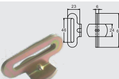
BTFTH007 BUTTERFLY FITTING FOR 25MM HOLE CAP: 909 kgs / 2,000 lb.
