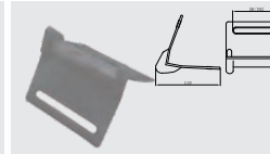
2"/4" White Plastic Corner Protector Weight=0.062kg
