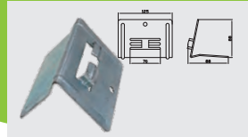
2"Corner Protector(Steel) Weight=0.304kg
