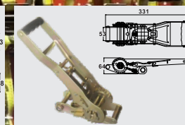
BTRB019 50MM ERGO, EXTRA LONG WIDE HANDLE CAP: 5,000 kgs
