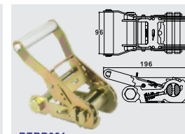
BTRB031 2" WITH WIDE HANDLE CAP: 7,000 kgs / 15,400 lbs.
