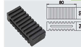
Tire Protector(Rubber or Plastic) 80MM×32 MM×24 MM
