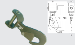
BTSF006 1-3/4" SWIVEL SNAP HOOK CAP: 3,500 kgs / 7,700 lbs.
