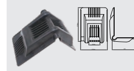
2"Black Corner Plastic Protector Weight=0.18kg
