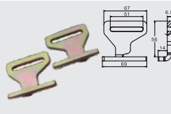
BTFTH003 LEFT HAND BTFTH004 RIGHT HAND 2" SPECIAL SLAT HOOK CAP: 1,363 kgs / 3,000 lbs.
