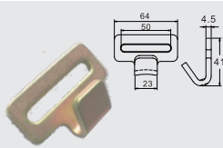
BTFTH005 2" SHORT NARROW FLAT HOOK CAP: 1,800 kgs / 3,960 lbs.
