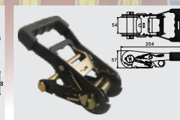
BTRB025 50MM WITH RUBBER HANDLE CAP: 5,454 kgs / 12,000 lbs.
