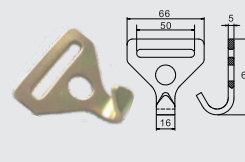
BTFTH001 2" F TRACK HOOK CAP: 1,000 kgs / 2,200 lbs.
