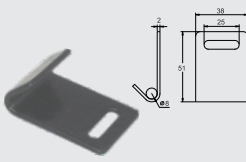
BTSF007 1" FLAT HOOK, PE COATING CAP: 500 kgs / 1,100 lbs.
