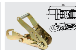
BTRB027 W/ F081-A CAP: 3,000 kgs/ 6,600 lbs BTRB028 W/ F082-A CAP: 5,000 kgs/ 11,000 lbs
