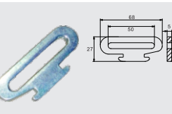
BTFTH010 TRACK FITTING CAP: 1,250 kgs / 2,750 lbs.
