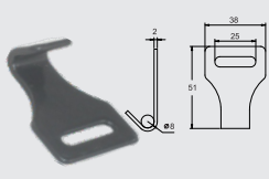
BTSF008 1" NARROW FLAT HOOK, PE COATING CAP: 450 kgs / 1,000 lbs.
