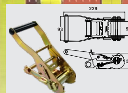
BTRB020 2" WITH PLASTIC HANDLE CAP: 5,000 kgs / 11,000 lbs.
