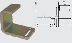
BTSF004 ROLL OFF HOOK CAP: 7,363 kgs / 16,200 lbs.
