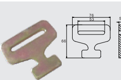
BTFTH011 T HOOK CAP: 3,182 kgs / 7,000 lbs.
