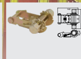
BTRB022 2" WRENCH-OPERATED CAP: 4,545 kgs / 10,000 lbs.
