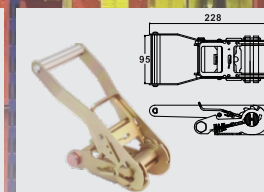
BTRB021 2" WITH ALUM LONG WIDE HANDLE CAP: 6,000 kgs / 13,200 lbs.
