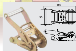
BTRB023 2" WITH ALUM MED. WIDE HANDLE CAP: 5,000 kgs / 11,000 lbs.
