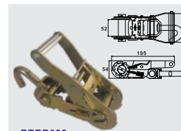
BTRB030 50MM WITH J HOOK CAP: 5,000 kgs
