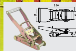
BTRb017 2" ERGO CAP: 5,000 kgs / 11,000 lbs.
