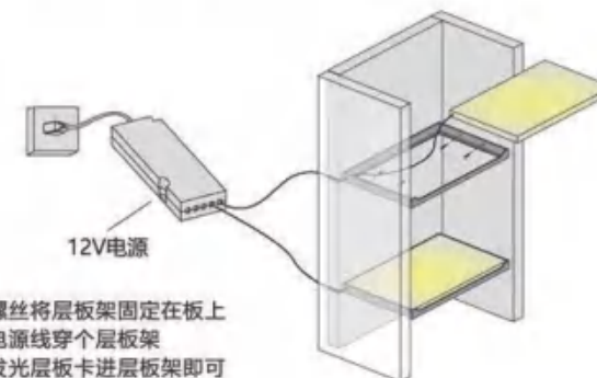
CURVED ARC MARBLE LUMINOUS LAMINATE NO. 15, 36MM THICK 36mm弯曲圆弧云石发光层板15号
