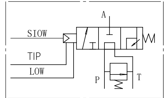
schematic diagram
