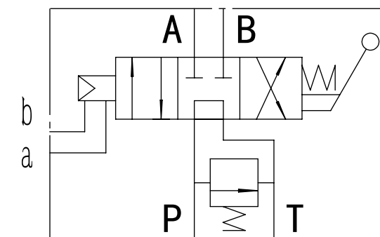
schematic diagram
