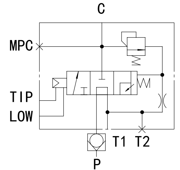
Hydraulic schematic diagram
