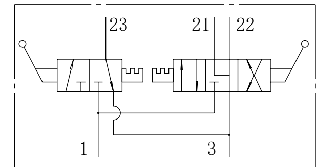
schematic diagram
