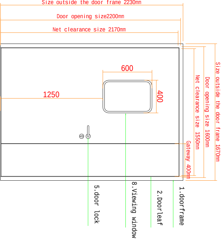
Elevation plan
