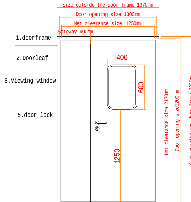
Elevation plan
