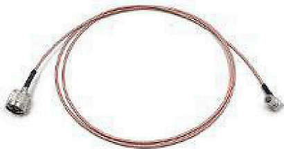
WDF-388 •QMA male R/A to N male for RG316 cable assembly
